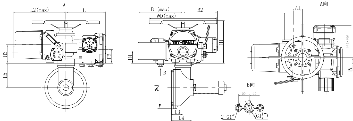
SMC-03Ex (IN) 带BA外形尺寸
